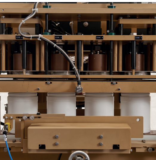
SHEMESH AUTOMATION'S SEALPRO120 FULLY AUTOMATIC LAMINATE CUTTING AND THERMO SEALING MACHINE WITH COMPLETE EXPLOSION (EX) AND CORROSION PROTECTION
